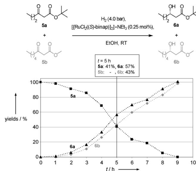
Figure 2. Progress with time of the AH of a 1:1 (mol/mol) mixture of \beta -ketoesters 5a and 5b ; ■ 5a , ▲ 6a , ◆ 6b . The progress was monitored by interrupting the reaction at the indicated times, removing an aliquot from the mixture (which was then resubmitted to AH conditions), and quantifying the amounts of reactants and products by GC (achiral capillary column) [23] by comparison with the reference peak. The reference was biphenyl, a known amount of which had been added to the reaction mixture at t = 0 h. t R ( 5a ) = 12.2 min, t R ( 6a ) = 13.6 min, t R ( 6b ) = 19.4 min, t R (biphenyl) = 27.3 min (1 \mu L, 55 °C (25 min)/20 K min -1 → 120 °C, p (H 2 ) = 60 kPa); the methyl ester 5b was not quantifiable in this way because of partial ethanolysis to 10 upon injection into the GC apparatus. [24]
