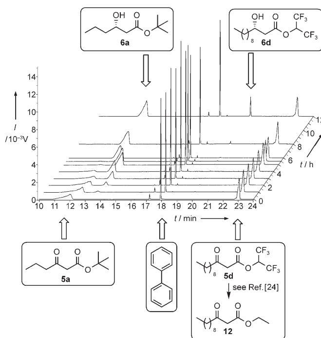
Figure 1. Gas-liquid chromatograms documenting the progress with time of the AH of the \beta -ketoester mixture shown in Figure 4.
