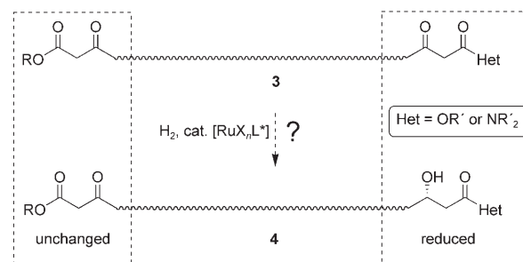
Scheme 2. Asymmetric monohydrogenation of bis( \beta -ketocarboxylic acid) derivatives 3 as a means of terminus differentiation.
