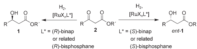
Scheme 1. Ru II -catalyzed AH of \beta -ketoesters 2 controlled by enantiomerically pure bisphosphane ligands. [1–3]
