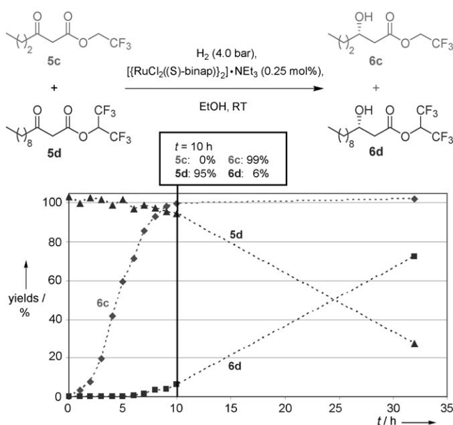
Figure 5. Progress with time of the AH of a 1:1 (mol/mol) mixture of \beta -ketoesters 5c and 5d ; \blacktriangle 5d , \blacktriangle 5d , \blacklozenge 6c , \blacksquare 6d . The yields were determined as detailed in Figure 2. The trifluoroethyl ester 5c was not quantifiable because of partial ethanolysis to 11 [24] upon injection into the GC apparatus; the hexafluoroisopropyl ester 5d was quantified as its ethanolysis product 12 [24] formed in the GC apparatus ( t_R(\text{12}) = 24.7 min); t_R(\text{6c}) = 11.1 min, t_R(\text{6d}) = 21.7 min, t_R(\text{biphenyl}) = 19.9 min (1 \mu\text{L} , 35 ^\circ\text{C} (15 min)/20 ^\circ\text{C min}^{-1} \rightarrow 140 ^\circ\text{C} (20 min), p(\text{H}_2) = 60 kPa).
