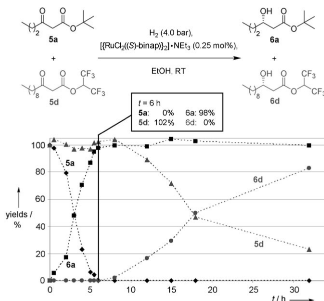
Figure 4. Progress with time of the AH of a 1:1 (mol/mol) mixture of \beta -ketoesters 5a and 5d ; \blacklozenge 5a , \blacktriangle 5d , \blacksquare 6a , \bullet 6d . The yields were determined as detailed in Figure 2. t_R(\mathbf{5a}) = 12.1 min; the hexafluoroisopropyl ester 5d was quantified as its ethanolysis product 12 [24] formed in the GC apparatus ( t_R(\mathbf{12}) = 23.0 min); t_R(\mathbf{6a}) = 13.5 min, t_R(\mathbf{6d}) = 19.9 min, t_R(\text{biphenyl}) = 17.9 min (1 \mu\text{L} , 55 ^\circ\text{C} (15 min)/20 ^\circ\text{C min}^{-1} \rightarrow 140 ^\circ\text{C} (10 min), p(\text{H}_2) = 60 kPa); see Figure 1 for the corresponding chromatograms.
