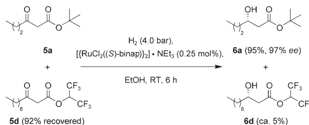
Scheme 3. Preparative-scale selective AH of the \beta -ketoester mixture shown in Figure 4 using 0.5 mmol of each reactant.
